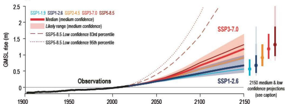
(a) Global mean sea level rise from 1900–2150
